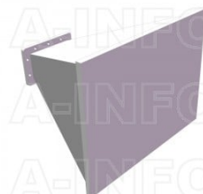
LB-510-15-ASPO Standard Gain Horn Antenna 1.45-2.2GHz 15dB Gain Rectangular Waveguide Interface
